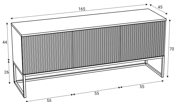
Cabinet 3 doors
